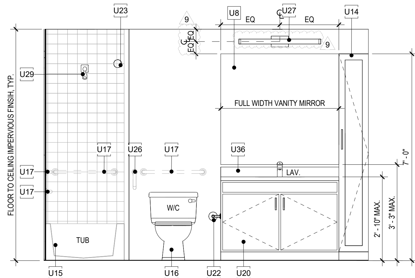
1 UNIT A1 BATHROOM EL. SCALE: 1/2" = 1'-0"
