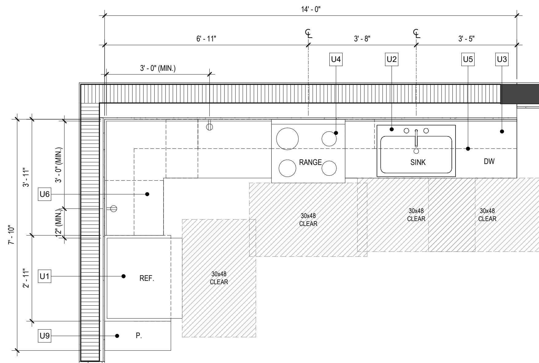
B UNIT A1 PLUMBING WALL KITCHEN PLAN SCALE: 1/2" = 1'-0"
