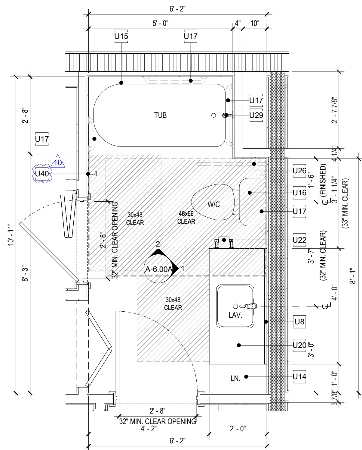
A UNIT A1 BATHROOM PLAN SCALE: 1/2" = 1'-0" TYPE A BATH
