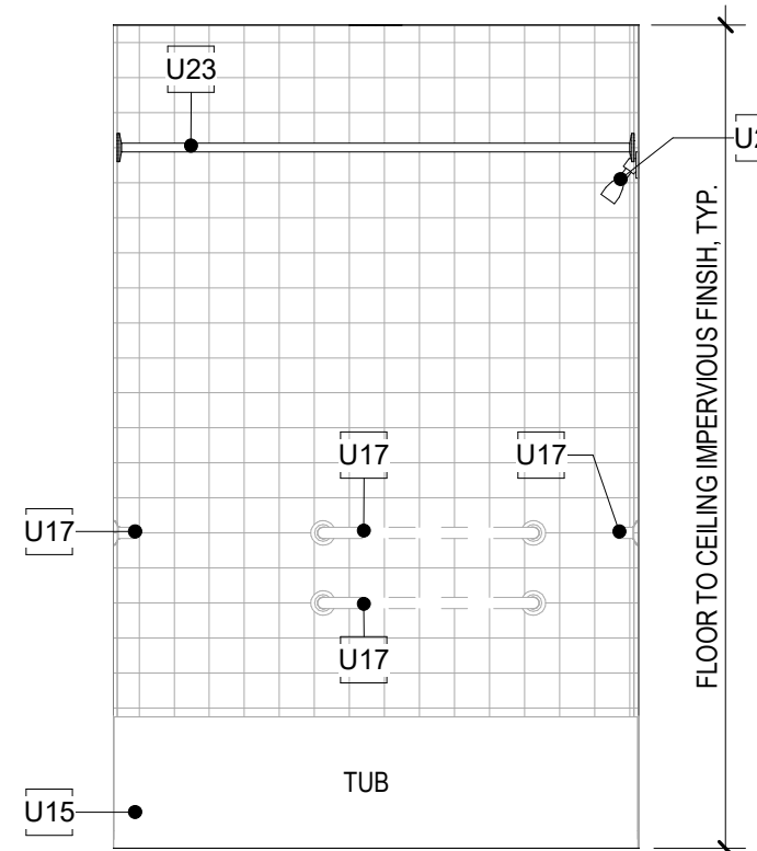
2 UNIT A1 BATHROOM EL. SCALE: 1/2" = 1'-0"
